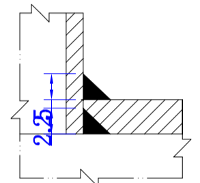
Details of the welding of the pipe and the barrel Not scaled
